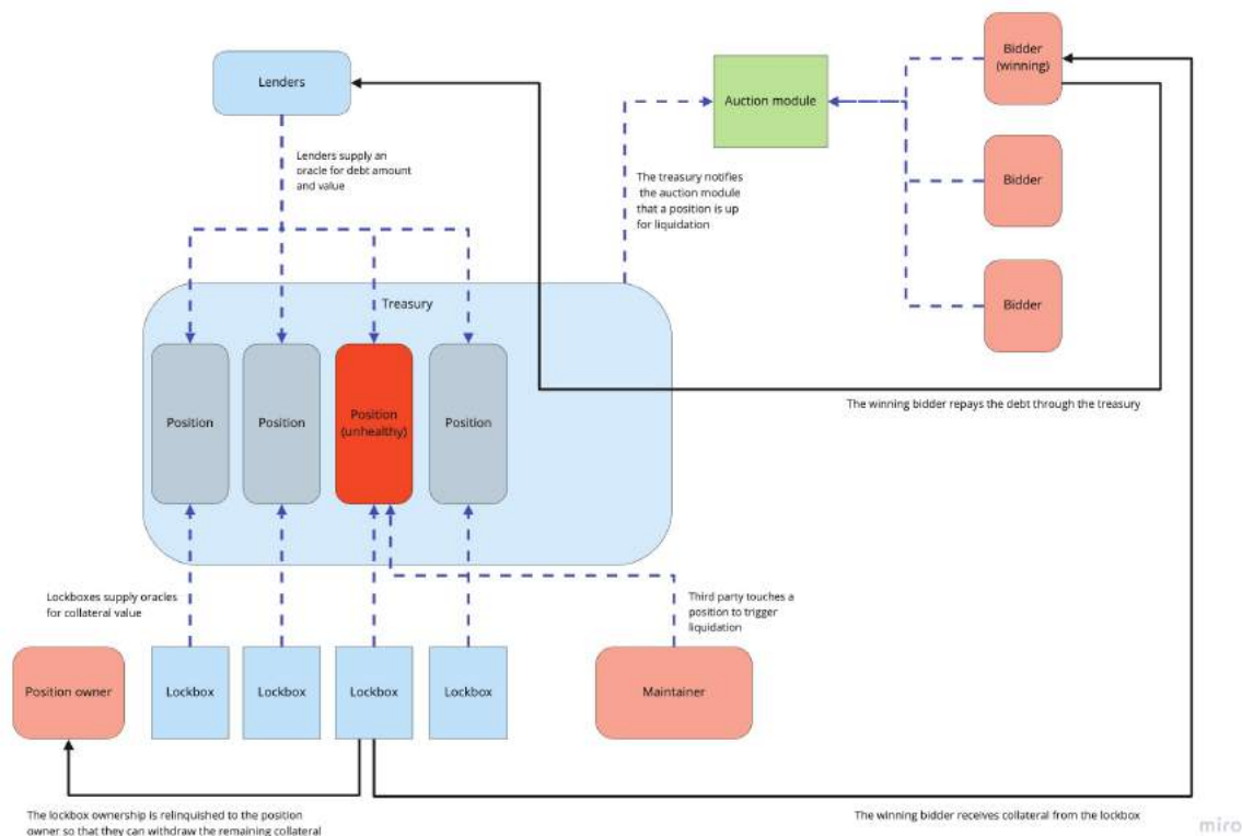
Figure 6: Alf Leverage liquidation flow. Blue lines indicate messages and black lines indicate value flows.
