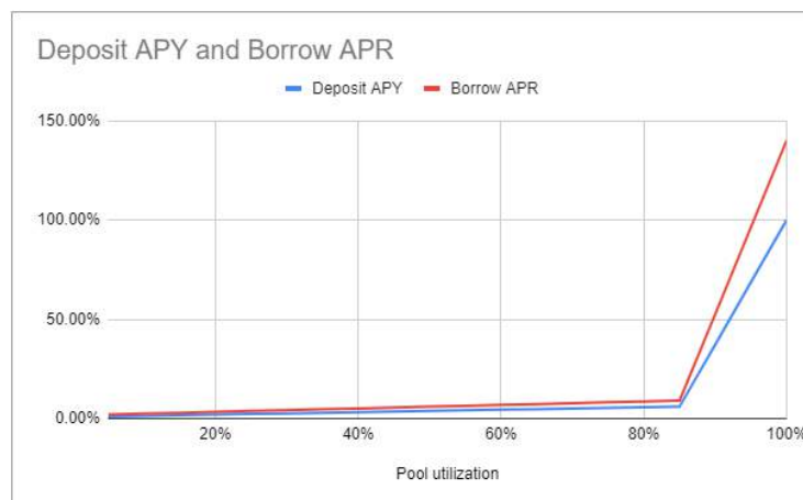
Figure 7: AAlf dynamic interest rate
