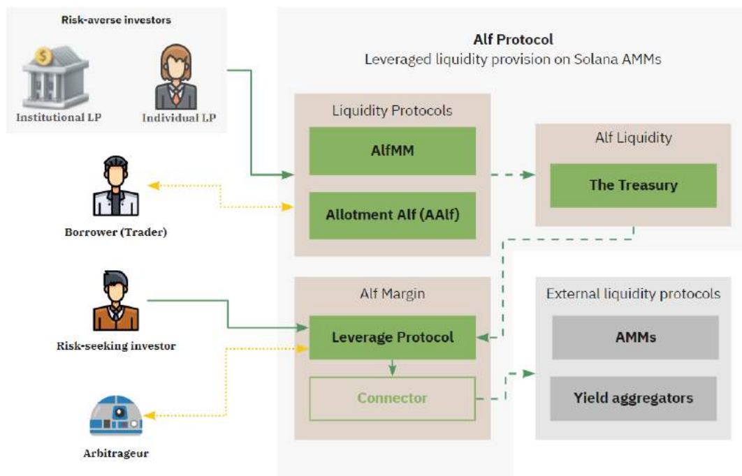
Figure 4: Cross-protocol liquidity facilitation by Alf.
